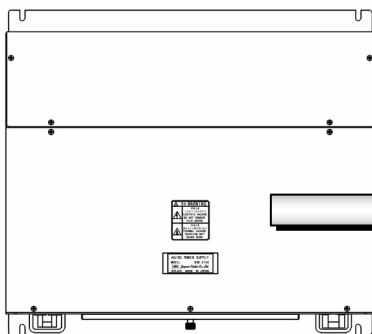
Ex) NBD-2150 AC/DC Power supply (Upper view)
